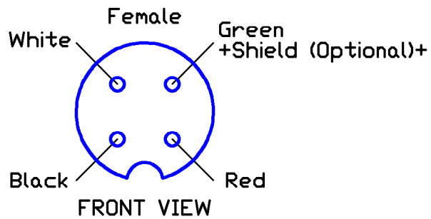
EN3P4F - Panel Connector (Controller Box) EN3L4F - InLine Cord Connector (Antenna Cable)
